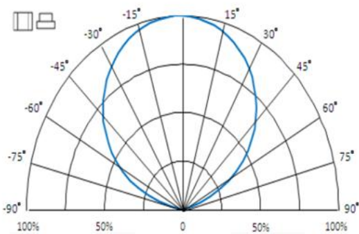
Directive Characteristics
