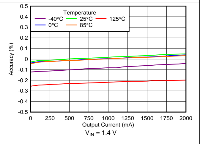
Figure 16. Load Regulation
