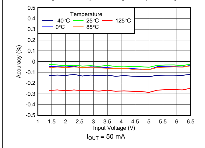
Figure 17. Line Regulation
