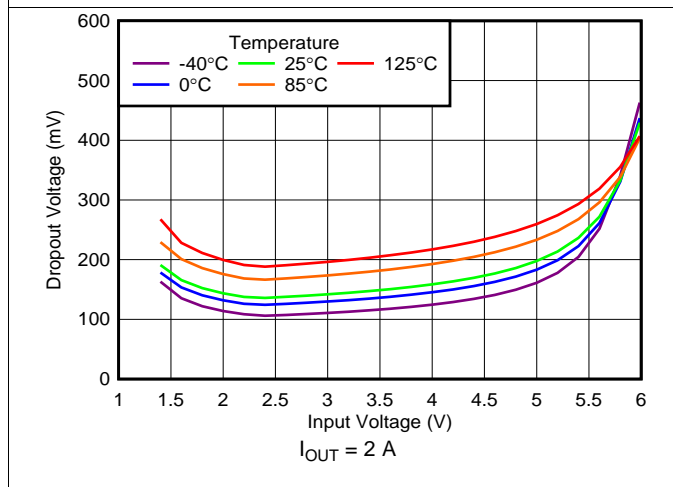
Figure 15. Dropout Voltage vs Input Voltage
