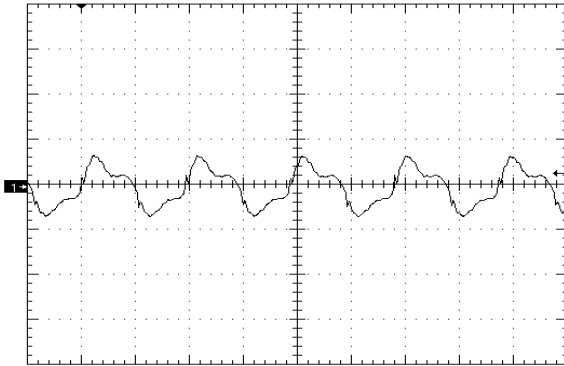
Figure 5. Output Voltage Ripple (50mV/div), time scale – 1uS/div. Vin=Vin_nom, full resistive Cout=1uF ceramic + 10uF Tantalum (see Fig 12)
