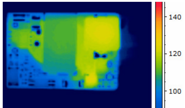
Figure 4. Thermal Image of CPT15A48 15A output, 55C Ambient, 100LFM, Vin = 48V, airflow from pin 3 to pin 1, T max = 121 °C)
