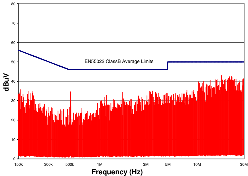
Figure 16. CPT15A48 Conducted Emissions using above specified input filter. Vin = 48V, Full Resistive Load
