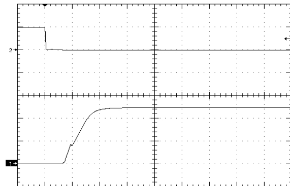
Figure 8. Startup Waveform via Enable Pin, time scale 10mS/div. Vin=Vin_nom, full resistive load + 4700uF, Ch1=2V/div, Ch2=5V/div
