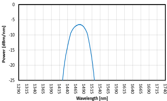
FIG. 5: SLED 4 SPECTRUM
