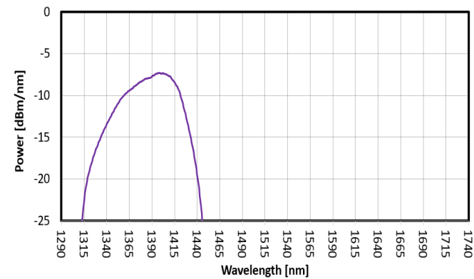
FIG. 6: SLED 5 SPECTRUM
