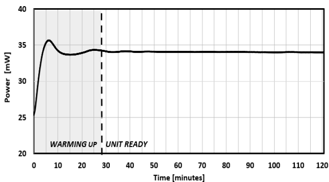
FIG. 13: WARM-UP TIME
