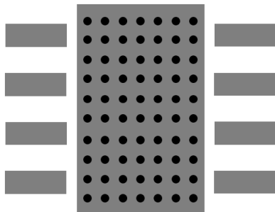
70 ground vias 0.008 inch finished hole diameter
