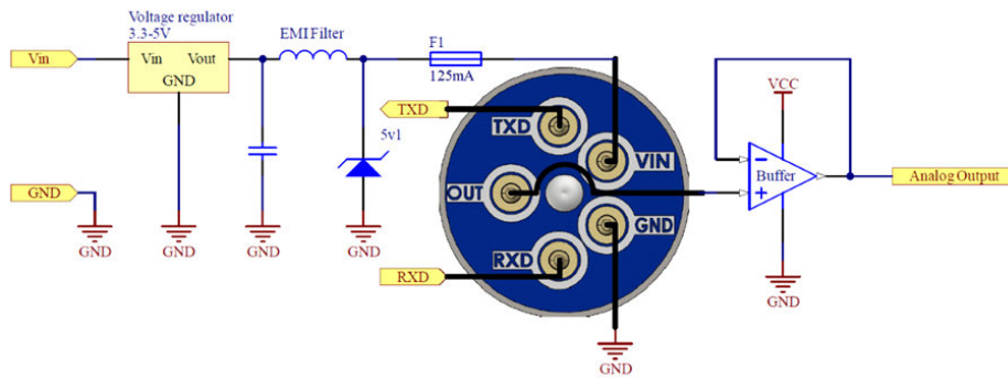
Fig.1 Example schematic for Interfacing Integrated IR (INIR2-ME100%)
