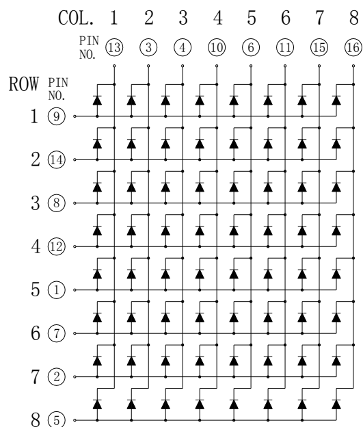
Common Row Anode: KWM-20881AVA
