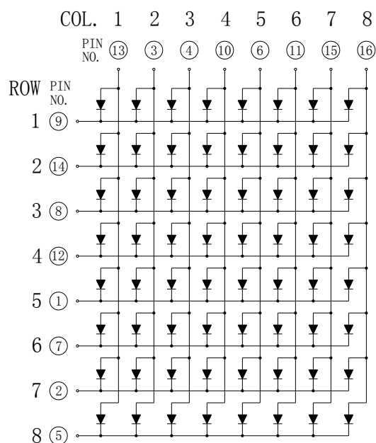
Common Row Cathode: KWM-20881CVA
