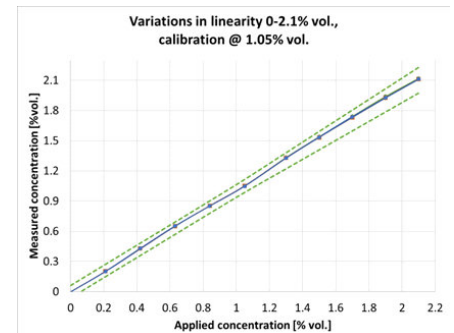
Typical Linearity 0-2.1% Propane
