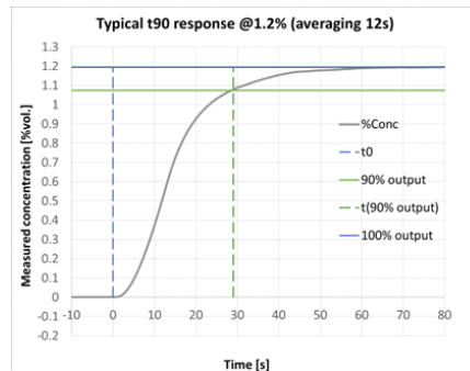
Typical T90 Response Time without Dust Filter (to 1.2% Propane)
