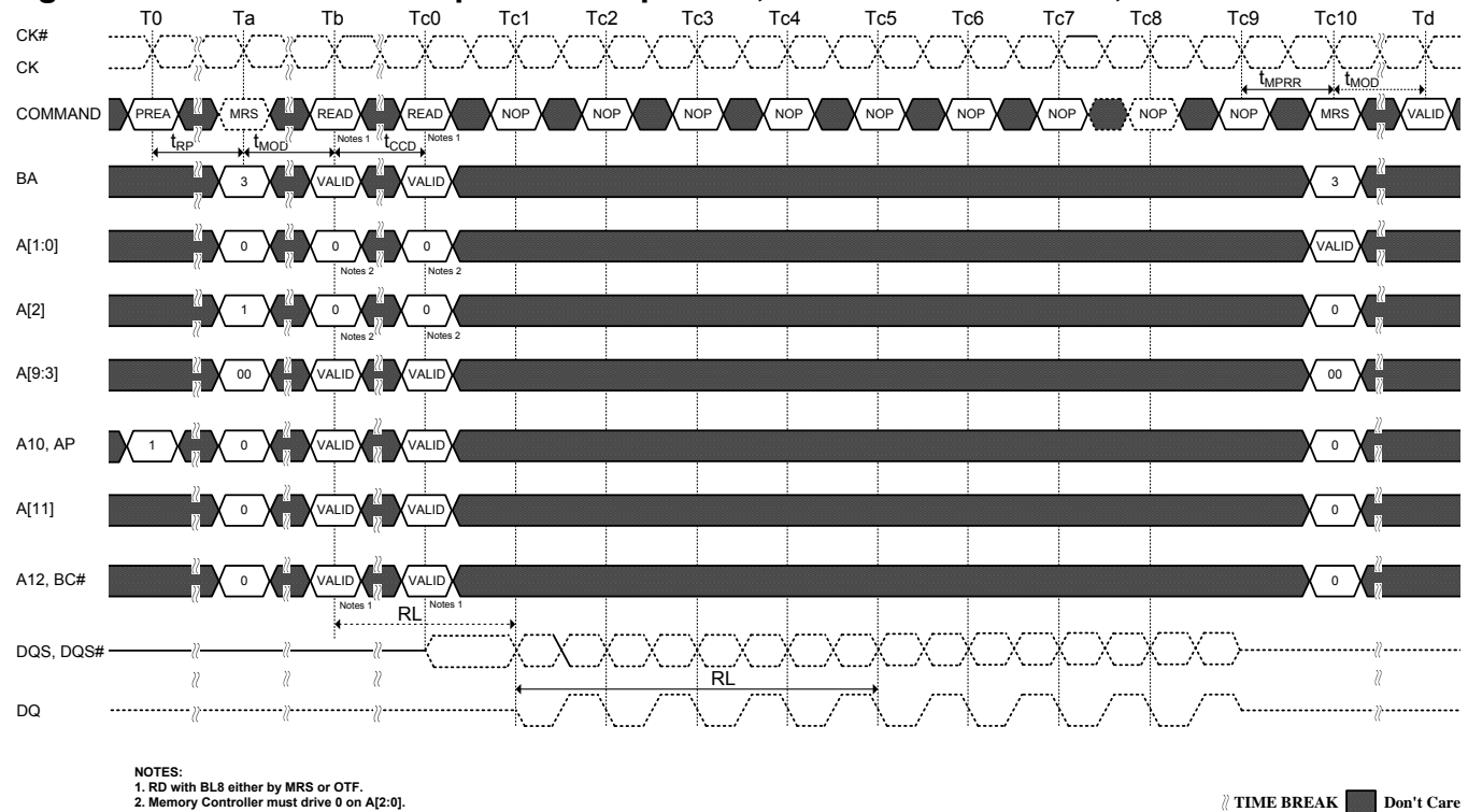
Figure 53. MPR Readout of predefined pattern, BL8 fixed burst order, back to back readout
