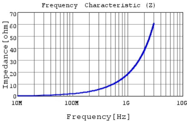
LQG15WZ2N9B02 |Z|
