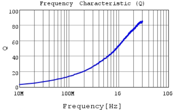
LQG15WZ2N9B02 Q
