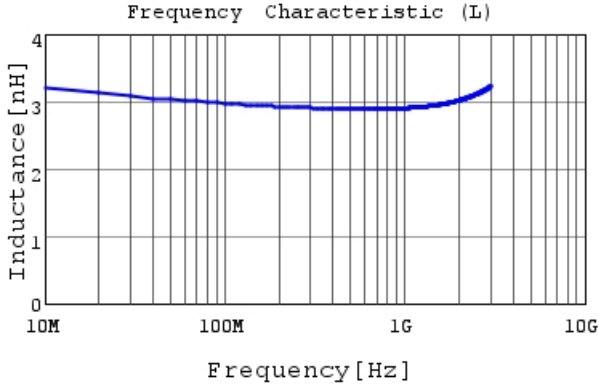
LQG15WZ2N9B02 L
