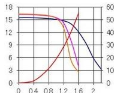
8. CDRH50D28BT150NP-150MC
