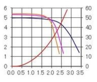
5. CDRH50D28BT150NP-4R7NC
