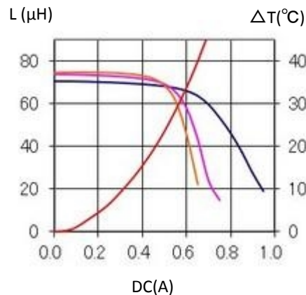
12. CDRH50D28BT150NP-680MC
