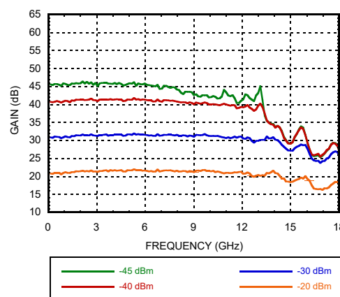
Response vs. Input Power [1][3][5]
