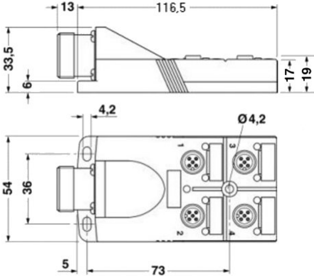
Dimensioned drawing
