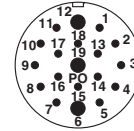
M23 plug connection pin, 19-pos.
