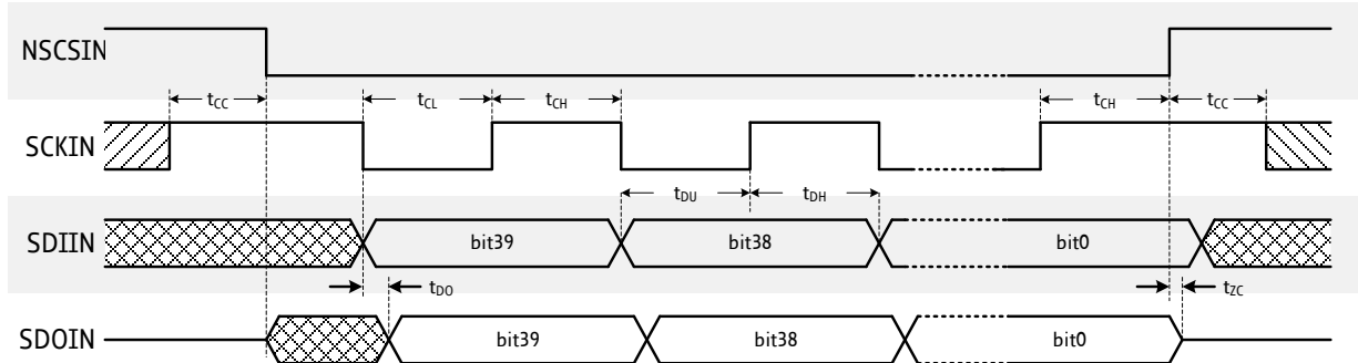
Figure 5.1 SPI timing
