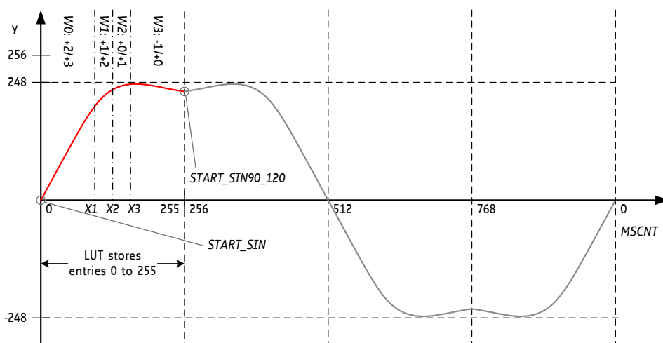
Figure 11.1 LUT programming example
