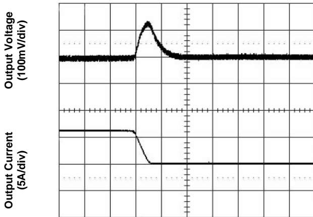
Figure 7. Transient Load Response (typical V_{in} , load current steps from 50% to 25% at a slew rate 0.1A/µs)
