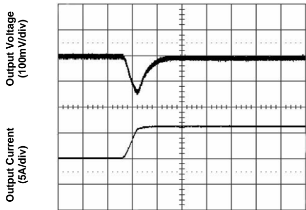
Figure 8. Transient Load Response (typical V_{in} , load current steps from 50% to 75% at a slew rate 0.1A/µs)
