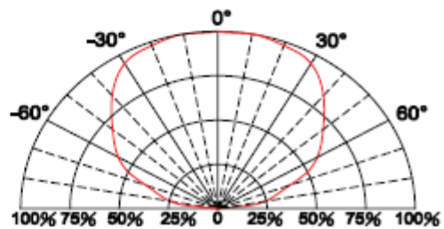
Fig.6 Directive Radiation
