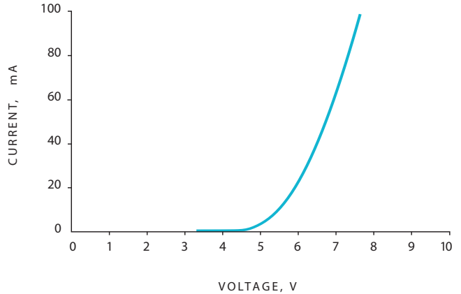
Electrical Characteristics
