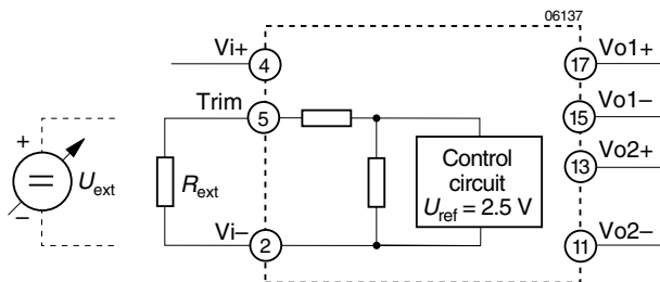
Fig. 14 Output voltage control for double output units by means of the Trim input on the primary side.
