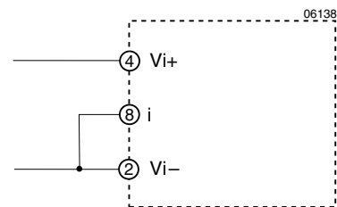
Fig. 22 If the inhibit is not used the inhibit pin should be connected to V_{i-}
