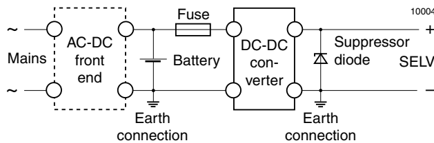
Fig. 20 Schematic safety concept. Use fuse, suppressor diode and earth connection as per table: Safety concept leading to an SELV output circuit.
