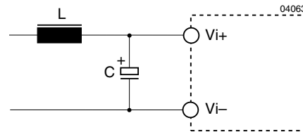
Fig. 5 Example for external circuitry to comply with IEC/EN 61000-4-5 or ETR 283 (19Pf11).
