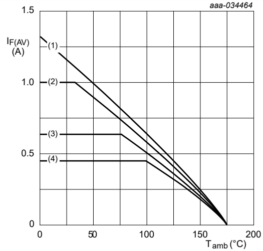
FR4 PCB, standard footprint T j = 175 °C (1) δ = 1; DC (2) δ = 0.5; f = 20 kHz (3) δ = 0.2; f = 20 kHz (4) δ = 0.1; f = 20 kHz
