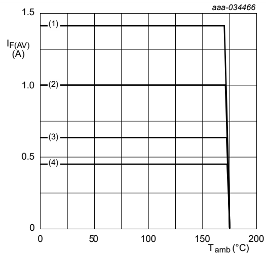
T j = 175 °C (1) δ = 1; DC (2) δ = 0.5; f = 20 kHz (3) δ = 0.2; f = 20 kHz (4) δ = 0.1; f = 20 kHz
