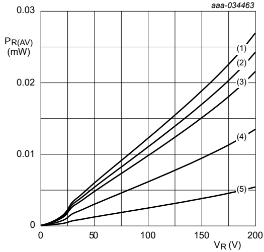
T j = 100 °C (1) δ = 1; DC (2) δ = 0.9 (3) δ = 0.8 (4) δ = 0.5 (5) δ = 0.2
