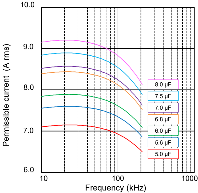
[ Permissible Current ]
