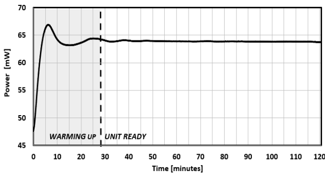
FIG. 9: WARM-UP TIME
