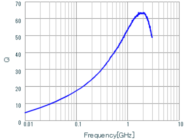
LQG15WZ9N1G02 Q.
