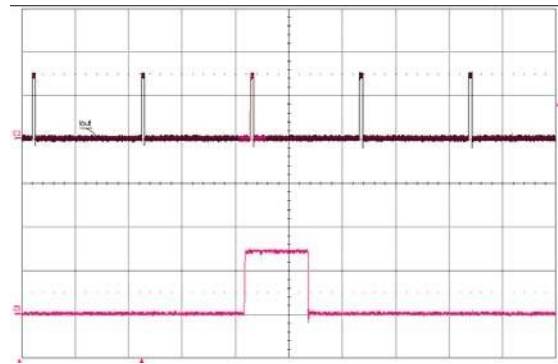
Figure 16. Load current (top trace, 20 A/div., 100 ms/div.) into a 10 m\Omega short circuit during restart, at V_{in} = 48 V. Bottom trace (20 A/div., 5 ms/div.) is an expansion of the on-time portion of the top trace.
