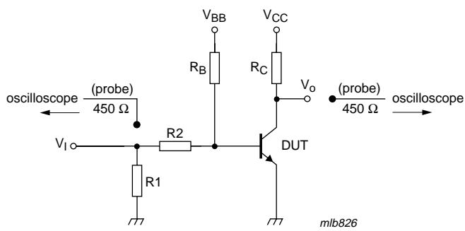
Fig 12. BISS transistor switching time definition
