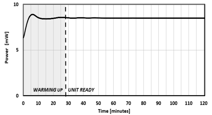
FIG. 4: WARM-UP TIME
