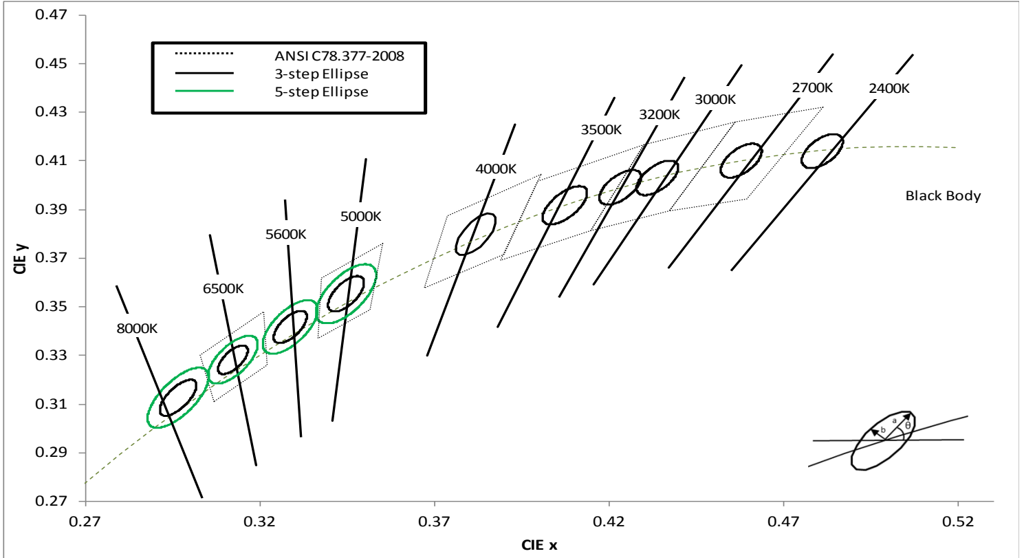
Chromaticity Bins: 1931 CIE Curve
