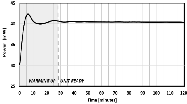
FIG. 15: WARM-UP TIME
