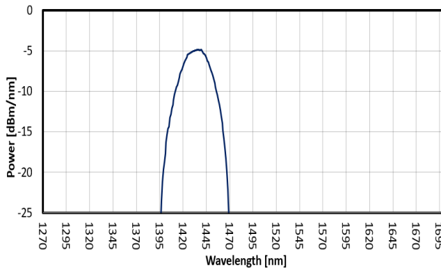
FIG. 5: SLED 4 SPECTRUM
