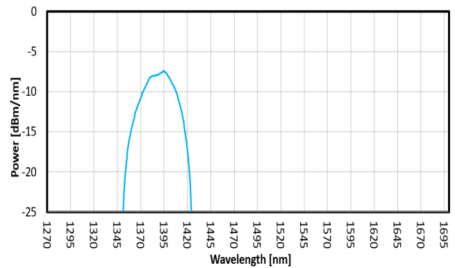
FIG. 6: SLED 5 SPECTRUM
