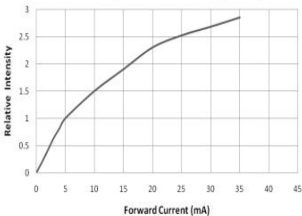
Relative Intensity VS. Forward Current (Ta=25°C)
