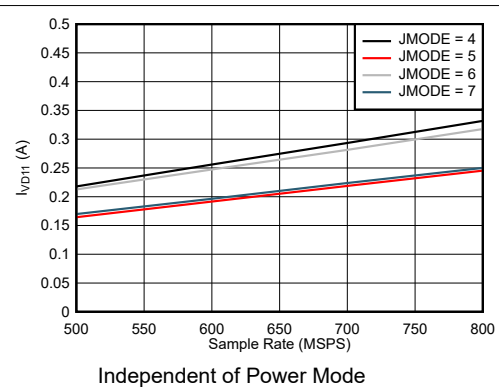
Figure 7-78. Quad Channel, I_{VD11} vs F_S for JMODES 4 - 7 Independent of Power Mode
