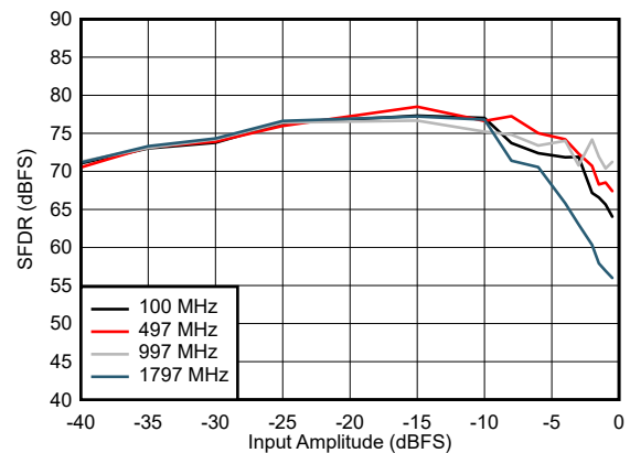
Figure 7-30. SFDR vs Input Amplitude
