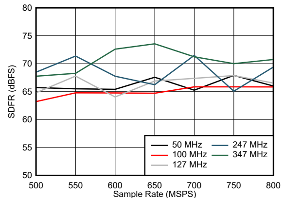
Low Power Mode Figure 7-24. SFDR vs Sample Rate
