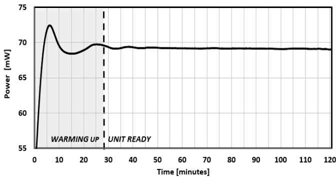
FIG. 9: WARM-UP TIME
