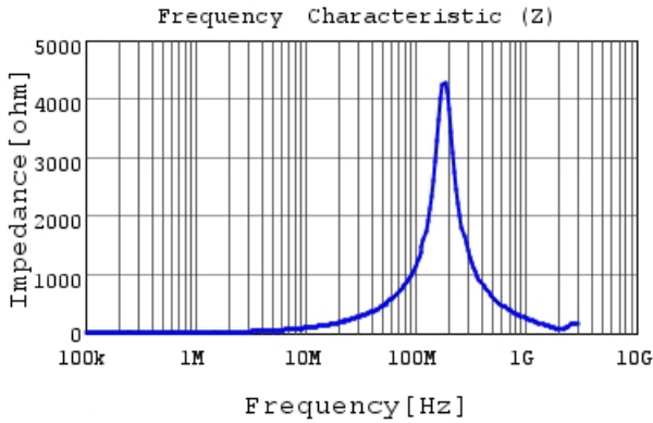
LQH32NZ1R5K23 |Z|
