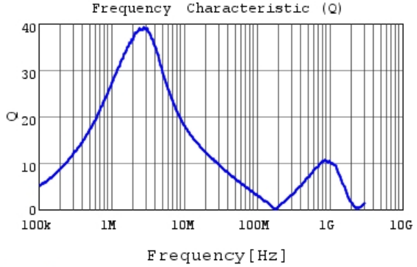
LQH32NZ1R5K23 Q
