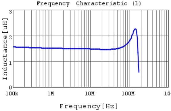
LQH32NZ1R5K23 L
