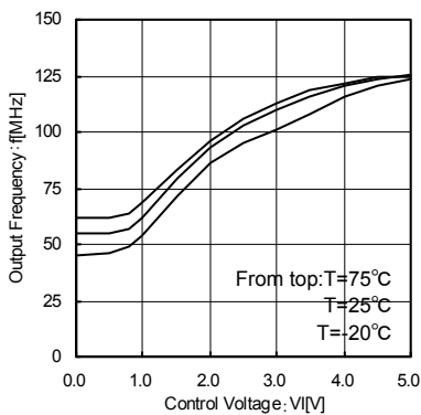
Fig.16 Control Voltage – Output Frequency (VDD=5.0V, Rbias=1.6KΩ)
