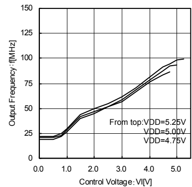
Fig.9 Control Voltage – Output Frequency (VDD=5.0V, Rbias=2.7KΩ, Ta=25°C)
