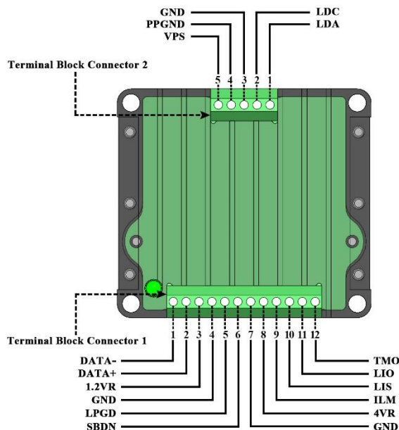
Figure 3. Top View of AQCL200MA410SE
