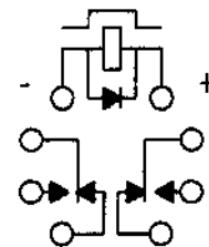
TERMINAL VIEW
