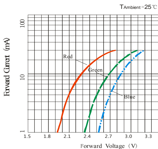
Volt-Ampere Characteristics
