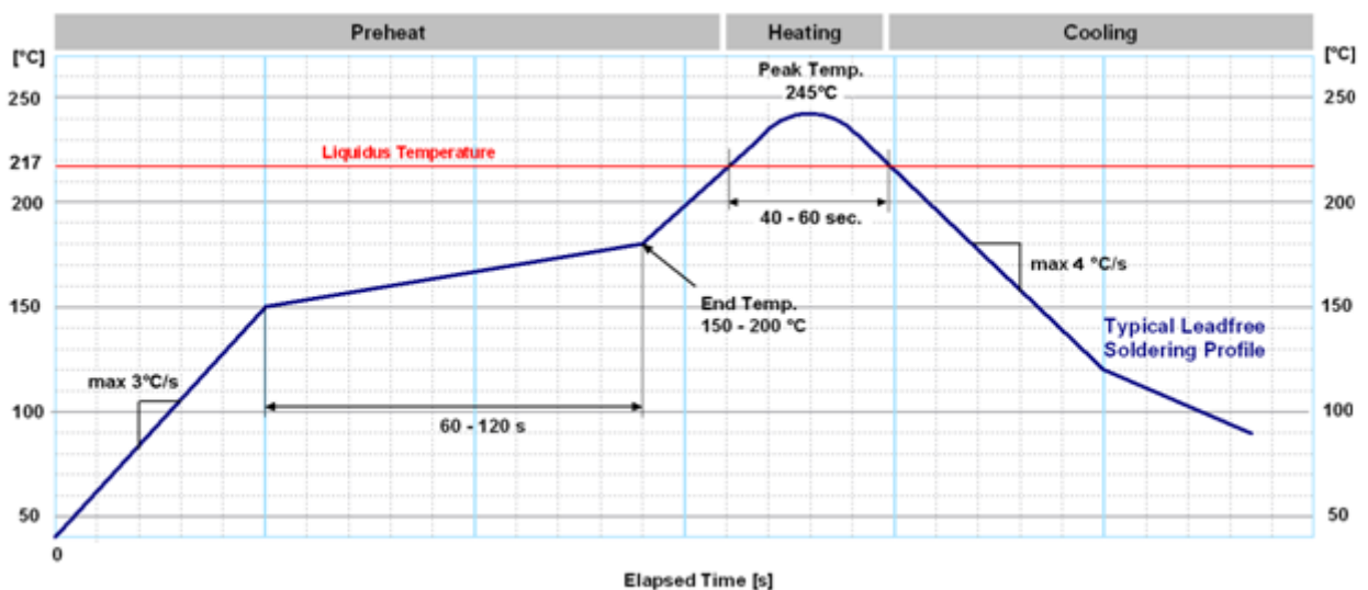
Figure 52: Soldering profile for professional grade ZED-F9P
