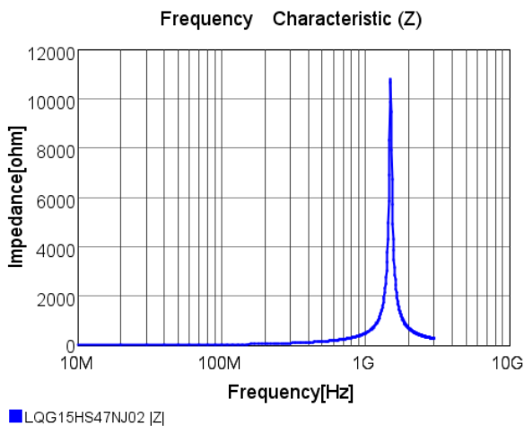
Figure 41: ZED-F9P antenna bias inductor impedance
