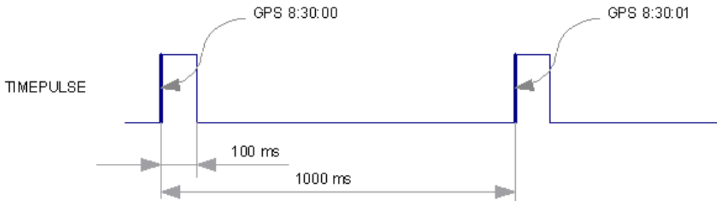
Figure 27: Time pulse signal with the example parameters
