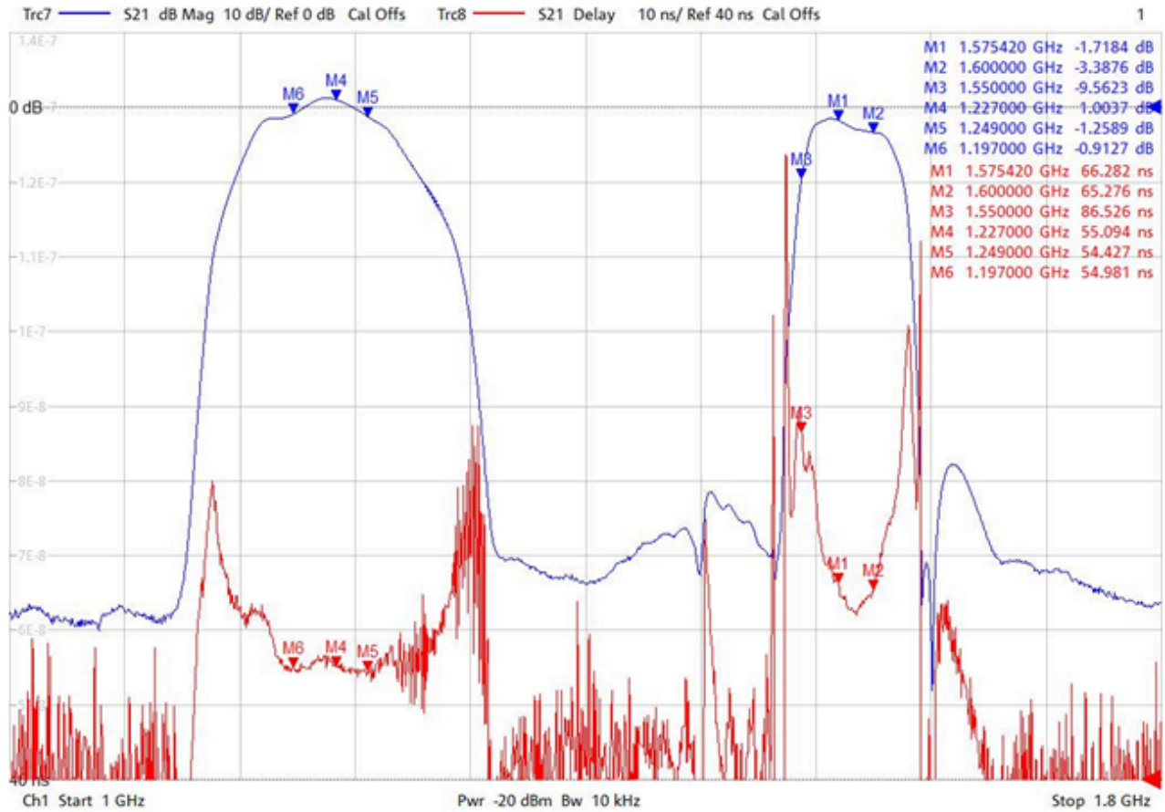
Figure 67: Low-cost L1/L2 antenna band characteristics
