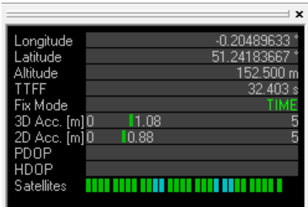
Figure 58: Base station: u-center data view in TIME mode
