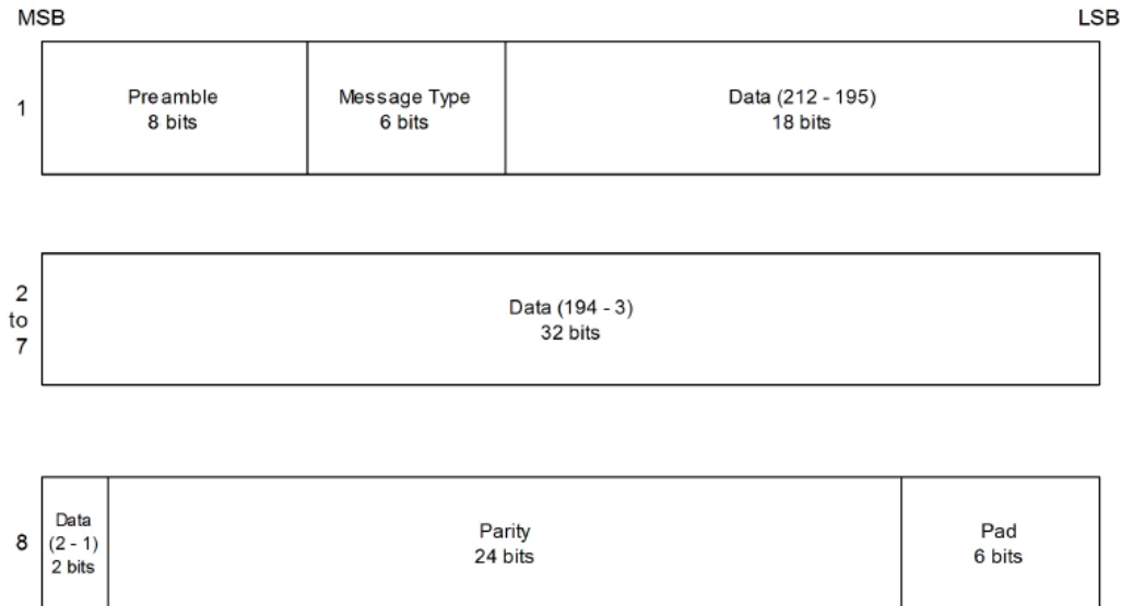
Figure 35: SBAS subframe words
