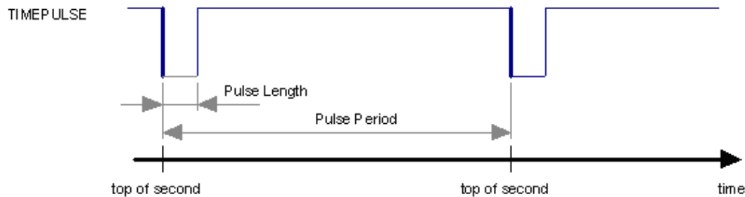
Figure 25: Time pulse
