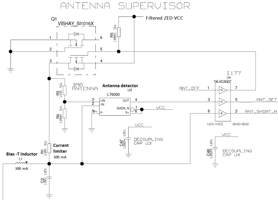
Figure 24: ZED-F9P antenna supervisor
