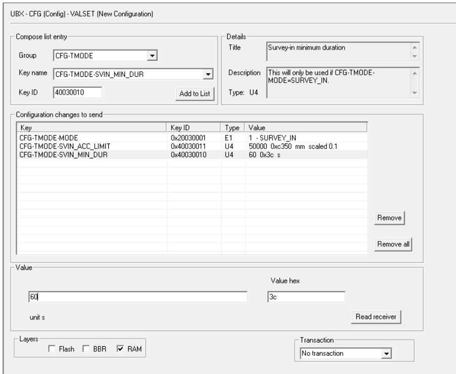
Figure 57: Base station: u-center UBX-CFG-VALSET message view for setting the CFG-TMODE-* configuration group required for performing a survey-in
