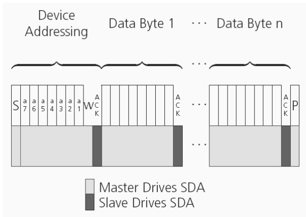
Figure 21: I2C write access
