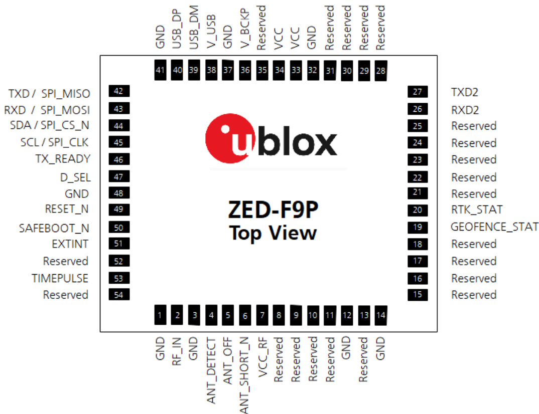
Figure 37: ZED-F9P pin assignment
