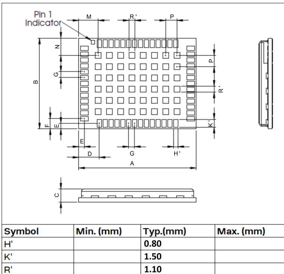
Figure 47: ZED-F9P suggested footprint (i.e. copper mask)
