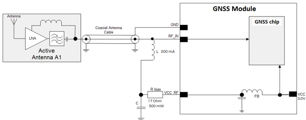
Figure 43: ZED-F9P VCC_RF antenna bias
