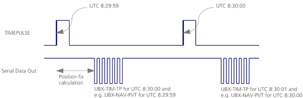
Figure 26: Time pulse and TIM-TP
