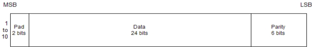
Figure 29: GPS L1C/A subframe word
