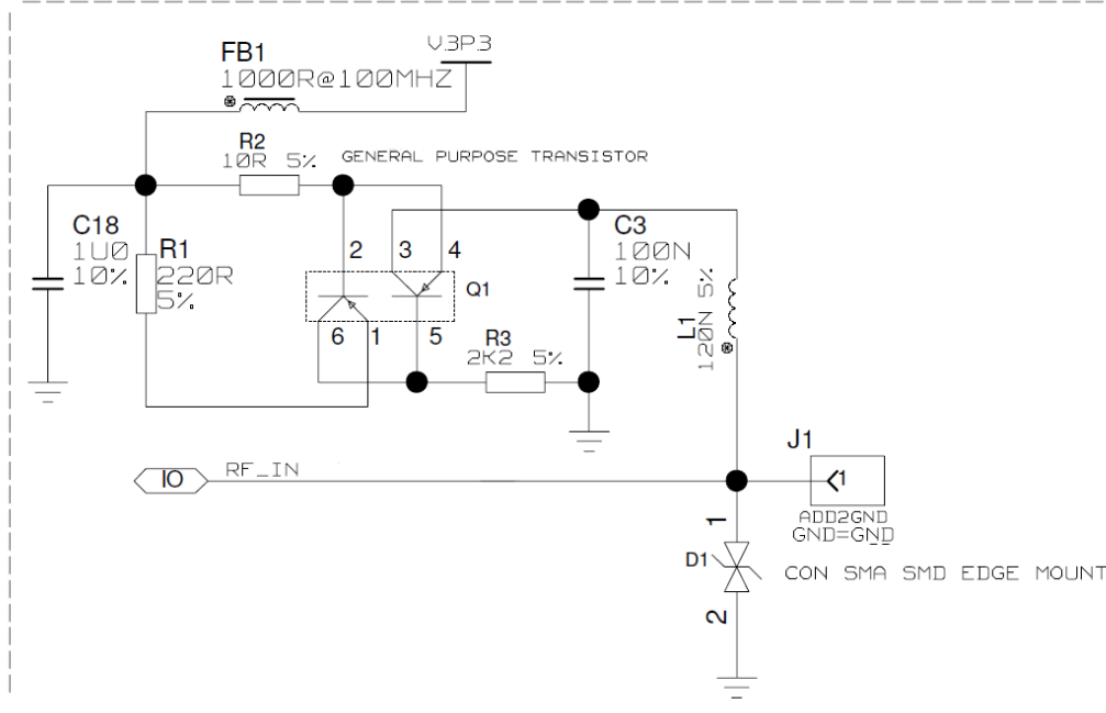
Figure 42: ZED-F9P reference design for antenna bias
