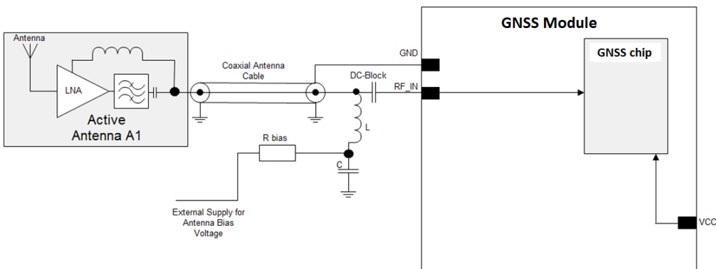
Figure 44: ZED-F9P external voltage antenna bias
