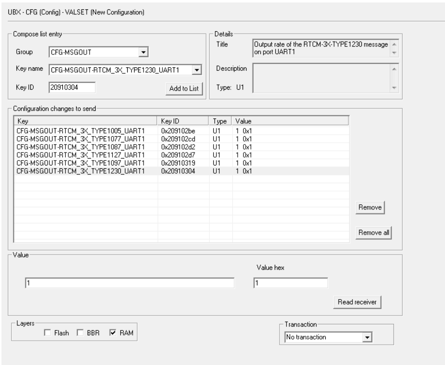
Figure 56: Base station: u-center UBX-CFG-VALSET message view for setting the CFG-MSGGOUT-* configuration group for enabling the output of the required RTCM messages
