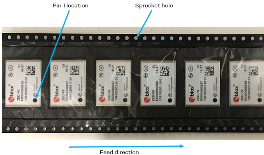
Figure 53: Orientation of ZED-F9P on the tape
