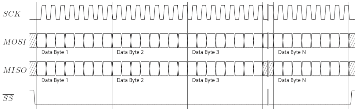
Figure 22: SPI back-to-back read/write access
