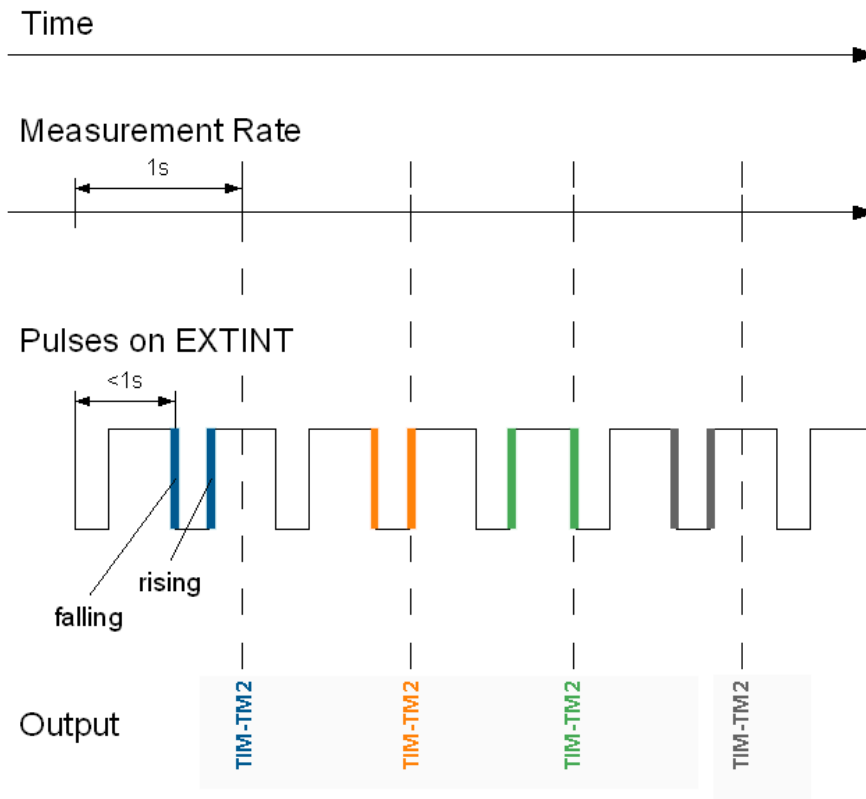
Figure 28: Time mark
