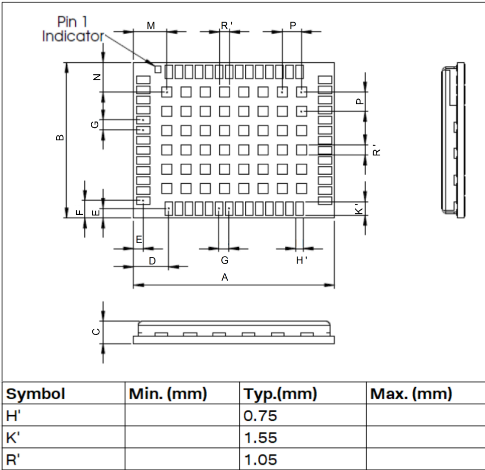
Figure 48: ZED-F9P suggested paste mask
