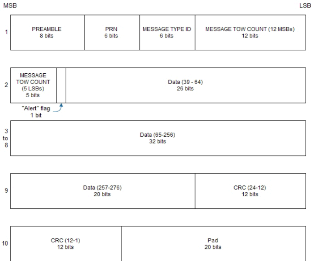
Figure 30: GPS L2C subframe words
