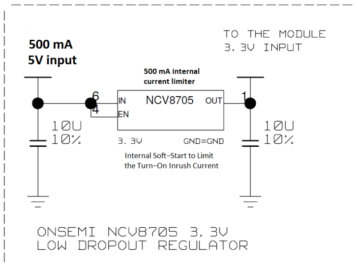
Figure 38: ZED-F9P power supply
