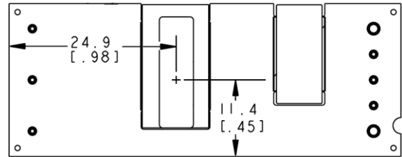
Figure 20. Pick and Place Location.
