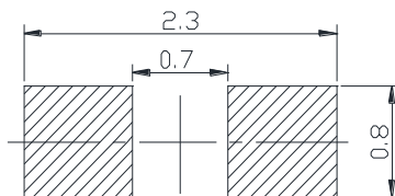
推荐焊盘尺寸 Recommended Soldering Pad
