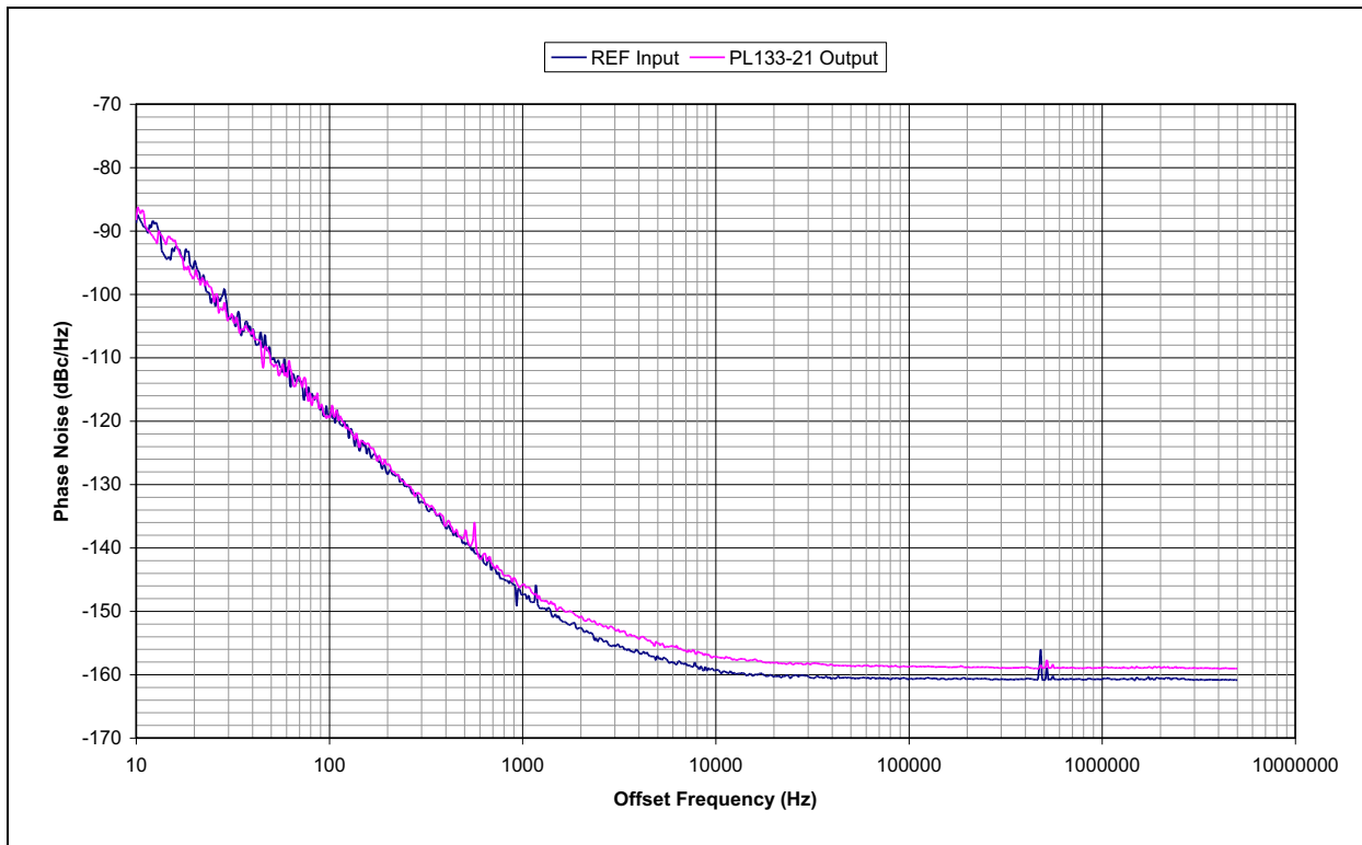
FIGURE 2-1: PL133-21 Additive Phase Jitter. V_{DD} = 3.3V , CLK = 26 MHz, Integration Range: 12 kHz to 5 MHz, 0.127 ps Typical.
